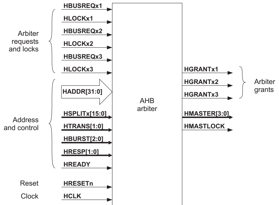
Figure 3-31 AHB arbiter interface diagram
