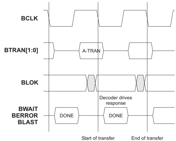
Figure 4-5 Address-only transfer
