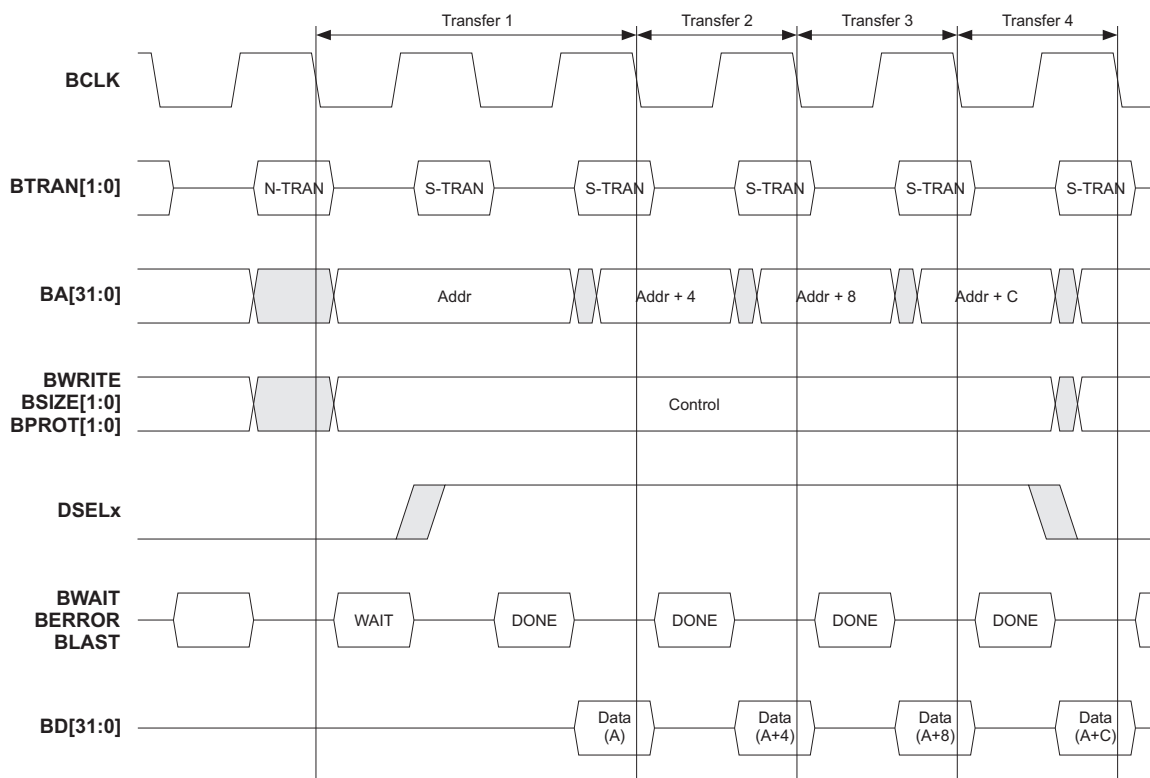
Figure 4-2 ASB transfers
