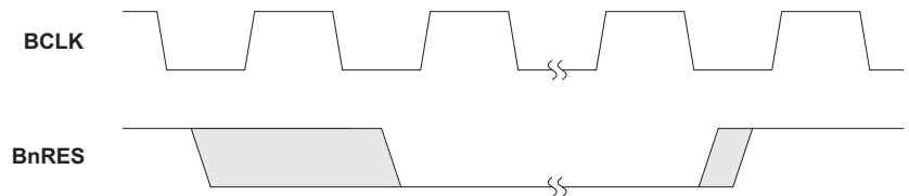
Figure 4-12 Reset signal
