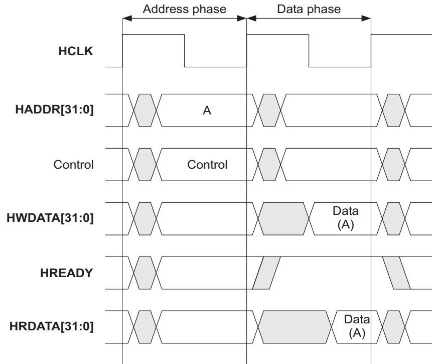
Figure 3-3 Simple transfer
