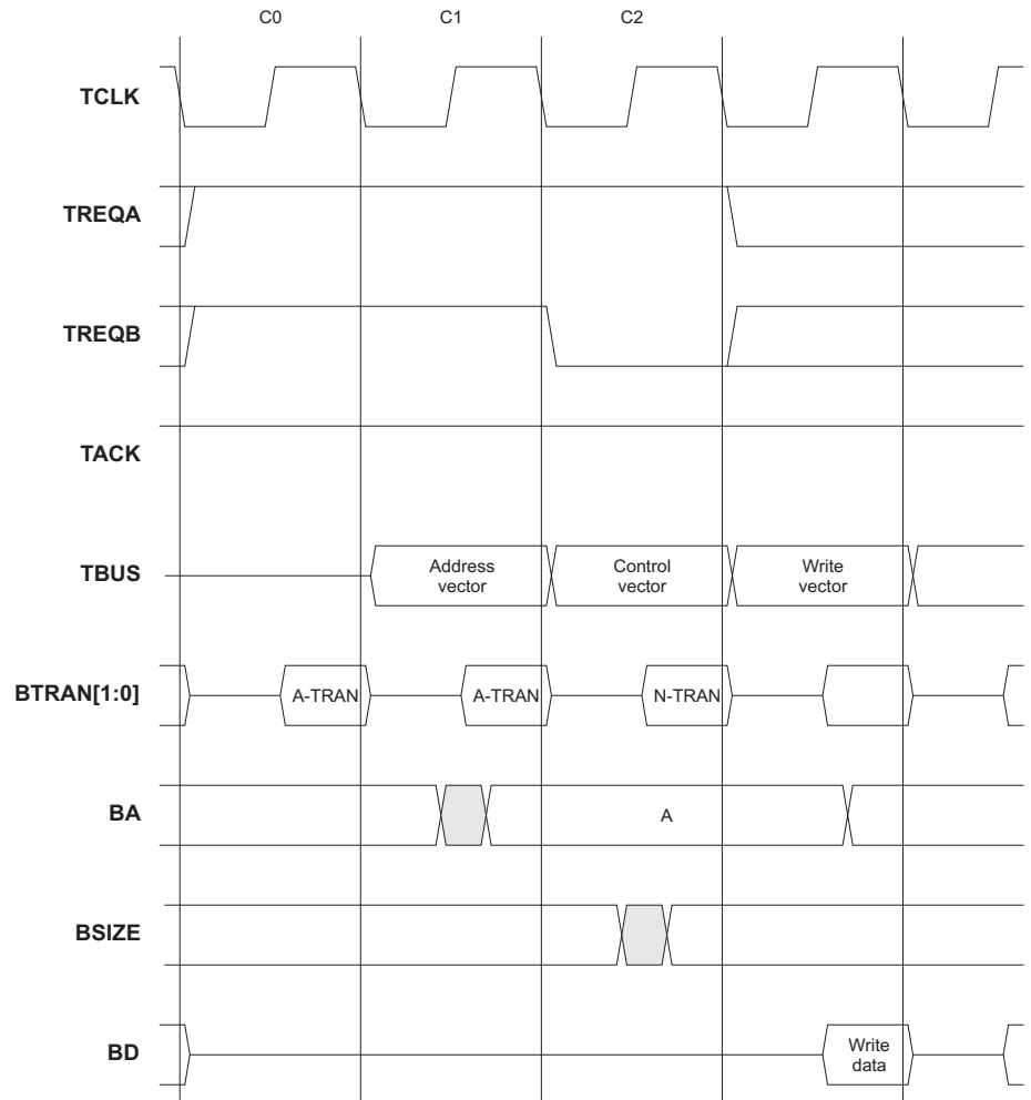
Figure 6-12 Control vector
