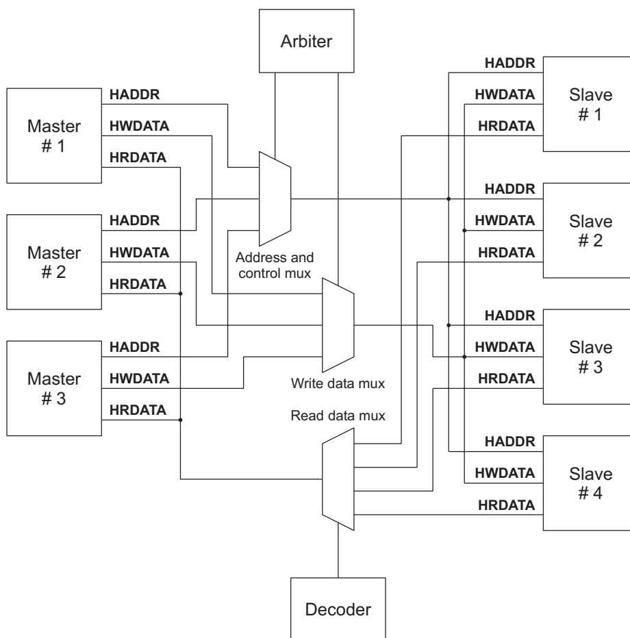
Figure 3-2 Multiplexor interconnection
