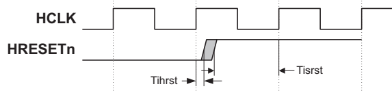
Figure 3-28 AHB master reset timing parameters
